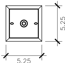
ELECTRIC MOUNTING PLATE
